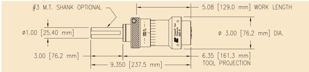
"AEX-2" SERIES ROLL-A-FINISH® TOOLS .062 TO 1.000 IN. (1.57 TO 25.4 MM)
